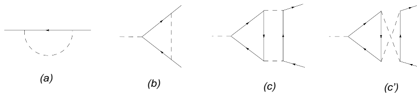
Figure 3: Subleading corrections.
